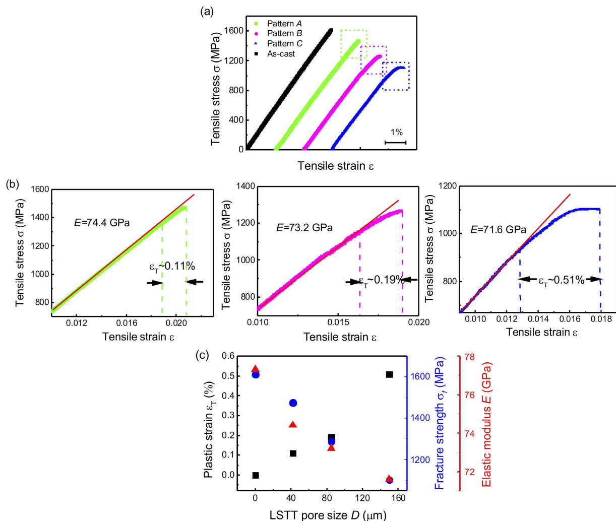
Figure 2. (a) Normal tensile stress-strain curves of un-LSTT (black) and LSTT samples (Green, magenta and blue). (b) The magnified parts of the tensile stress-strain curves in (a) circled by the green, magenta and blue dashed rectangular circles. (c) Variation of tensile plastic strain \epsilon_T , nominal fracture strength \sigma_f and elastic modulus E with different pore sizes. The value of elastic modulus is measured by fitting the elastic part of the tensile stress-strain curve.
