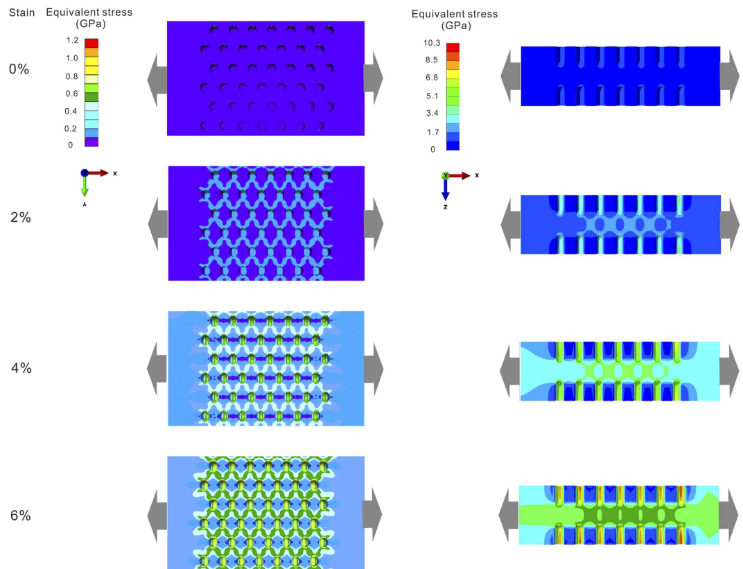
Figure 6. Equivalent stress distribution evolution of LSTT specimen with pore size 150\ \mu\text{m} at different tensile elastic strains (from top to down): 0%, 2%, 4% and 6%. The left graphs are the plan view and the right ones gives the cross-sectional view. The grey arrows give the tensile loading direction.
