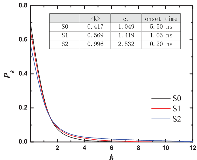
FIG. 7. Probability distribution of degree of bcc-like clusters in three samples. The inset table shows the average value of connectivity c and degree ( k ) of bcc-like clusters and the onset time of crystallization.
